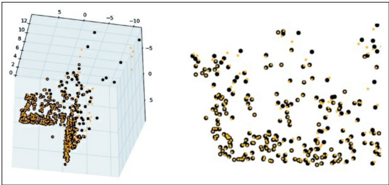
Figure 5-5. Triangulated points using camera matrices and point correspondences. The estimated points are shown with dark circles and the true points with light dots. View from above and to the side (left). Closeup of the points from one of the building walls (right).
