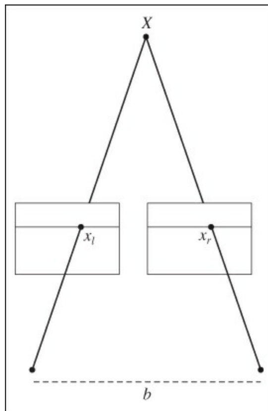
Figure 5-9. An illustration of a rectified stereo image setup where corresponding points are on the same row in both images.
