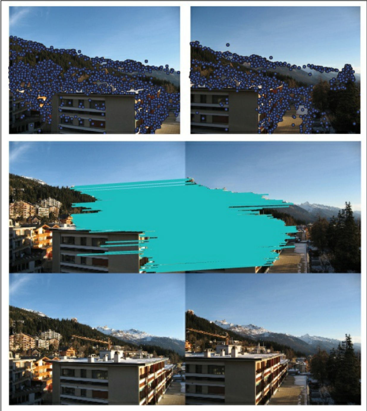
Figure 2-5. An example of detecting and matching SIFT features between two images.
