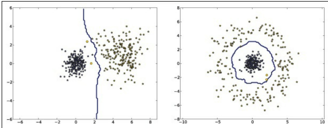
Figure 8-1. Classifying 2D data using a k-nearest neighbor classifier. For each example, the color shows the class label. Correctly classified points are shown with stars and misclassified points with circles. The curve is the classifier decision boundary.
