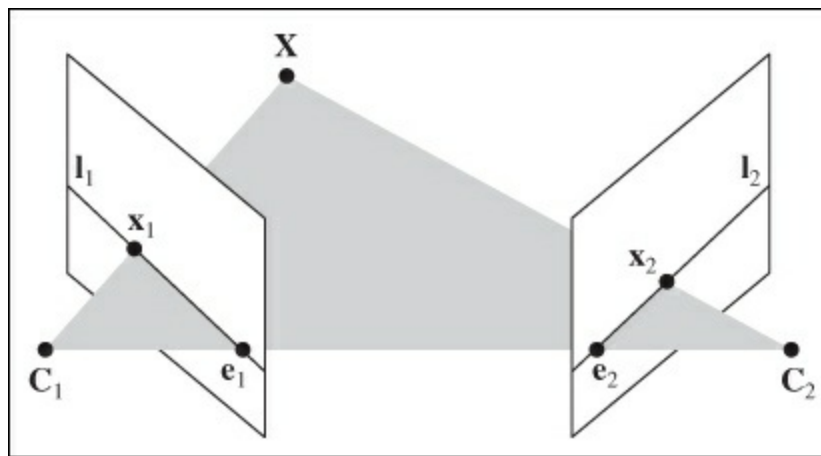
Figure 5-1. An illustration of epipolar geometry. A 3D point X is projected to x_1 and x_2 , in the two views, respectively. The baseline between the two camera centers, C_1 and C_2 , intersect the image planes in the epipoles, e_1 and e_2 . The lines l_1 and l_2 are called epipolar lines.
