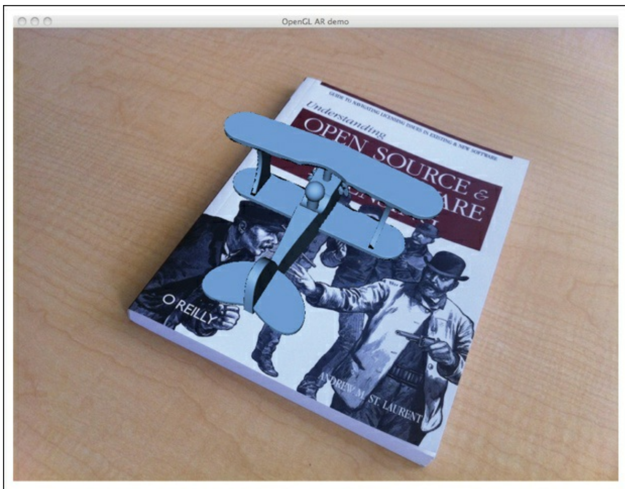
Figure 4-6. Loading a 3D model from an .obj file and placing it on a book in a scene using camera parameters computed from feature matches.
