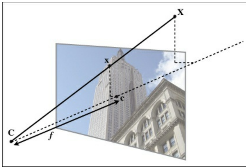
Figure 4-1. The pin-hole camera model. The image point x is at the intersection of the image plane and the line joining the 3D point X and the camera center C . The dashed line is the optical axis of the camera.
