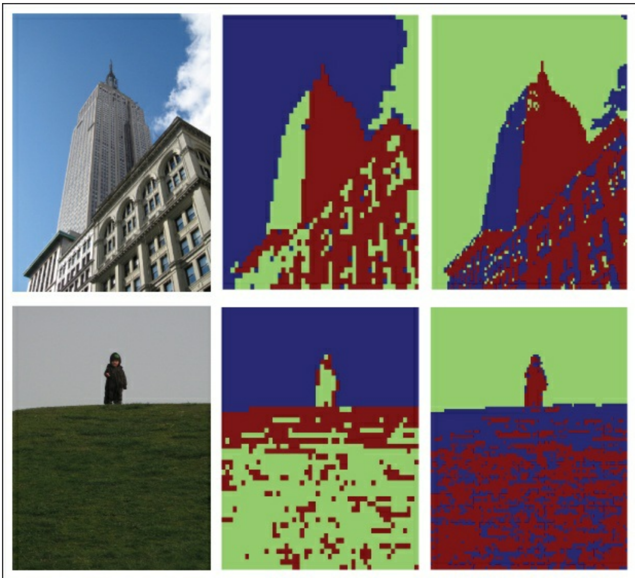
Figure 6-4. Clustering of pixels based on their color value using k-means: original image (left); cluster result with k = 3 and 50 \times 50 resolution (middle); cluster result with k = 3 and 100 \times 100 resolution (right).
