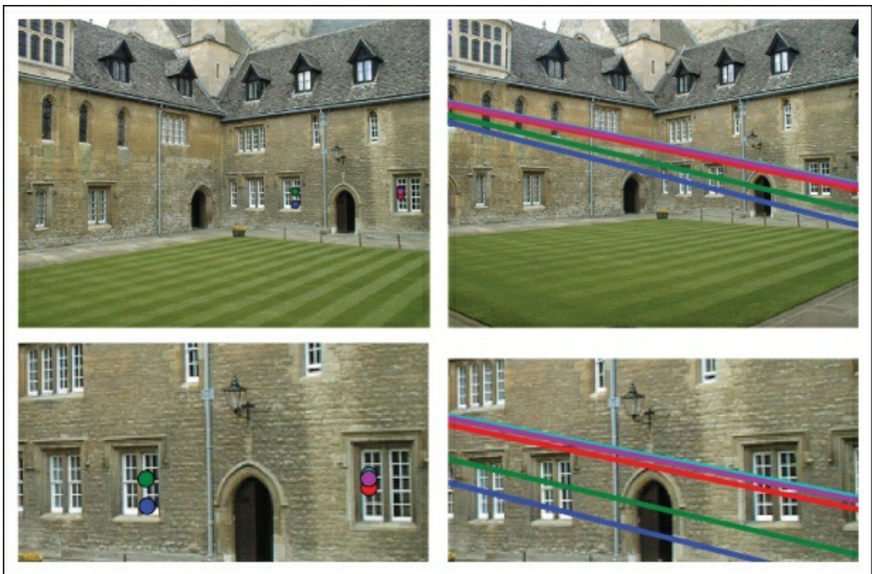
Figure 5-4. Epipolar lines in view 1 shown for five points in view 2 of the Merton1 data. The bottom row shows a closeup of the area around the points. The lines can be seen to converge on a point outside the image to the left. The lines show where point correspondences can be found in the other image (the color coding matches between lines and points).
