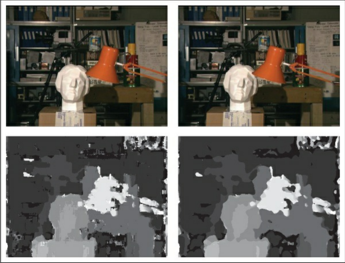
Figure 5-10. Example of computing disparity maps from a stereo image pair with normalized cross-correlation.
