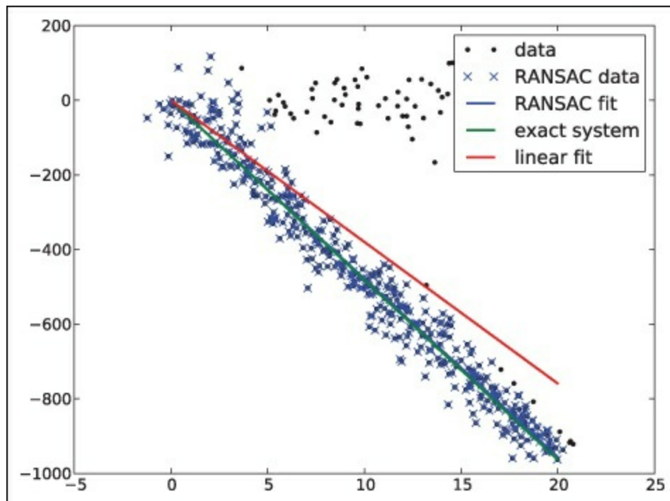
Figure 3-10. An example of using RANSAC to fit a line to points with outliers.
