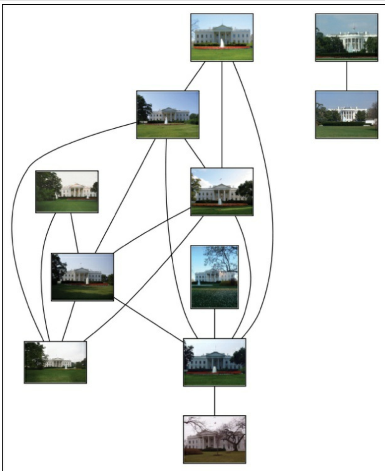
Figure 2-10. An example of grouping images taken at the same geographic location using local descriptors.
