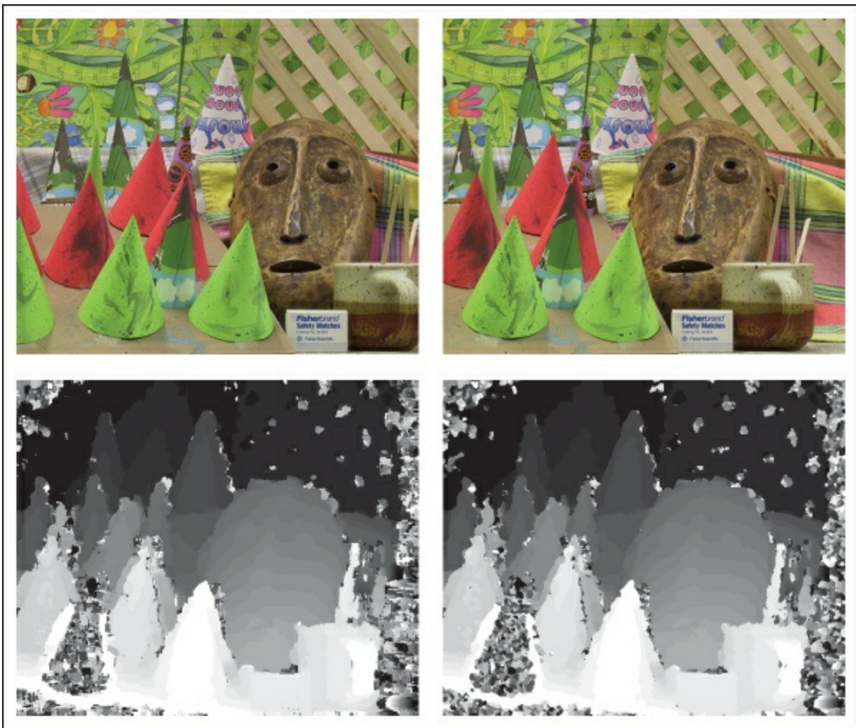
Figure 5-11. Example of computing disparity maps from a stereo image pair with normalized cross-correlation.
