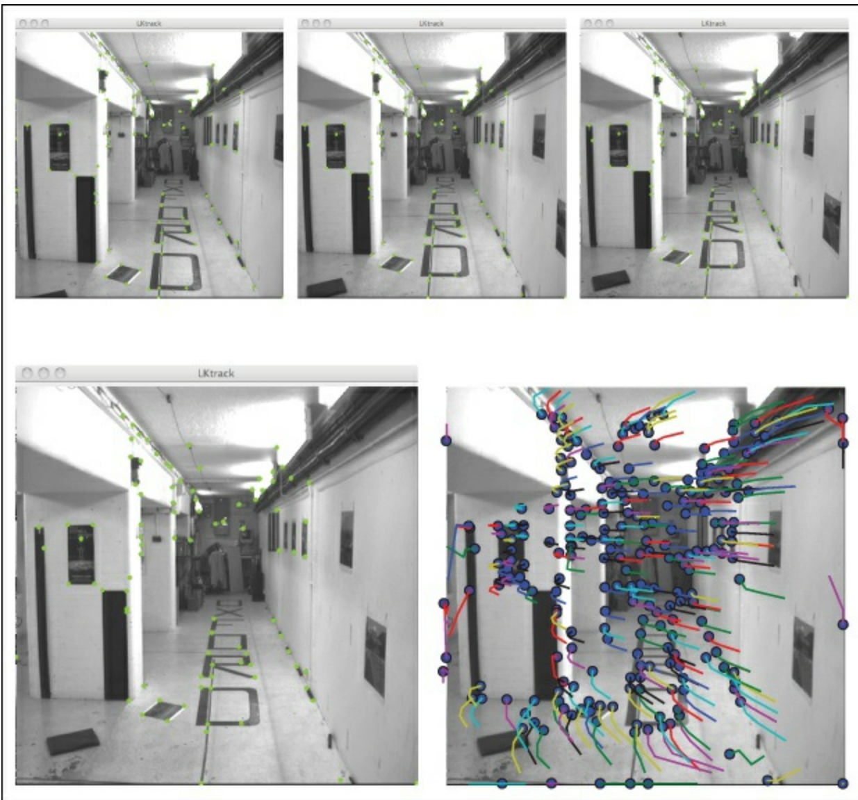
Figure 10-6. Tracking using the Lucas-Kanade algorithm through the LKTrack class.
