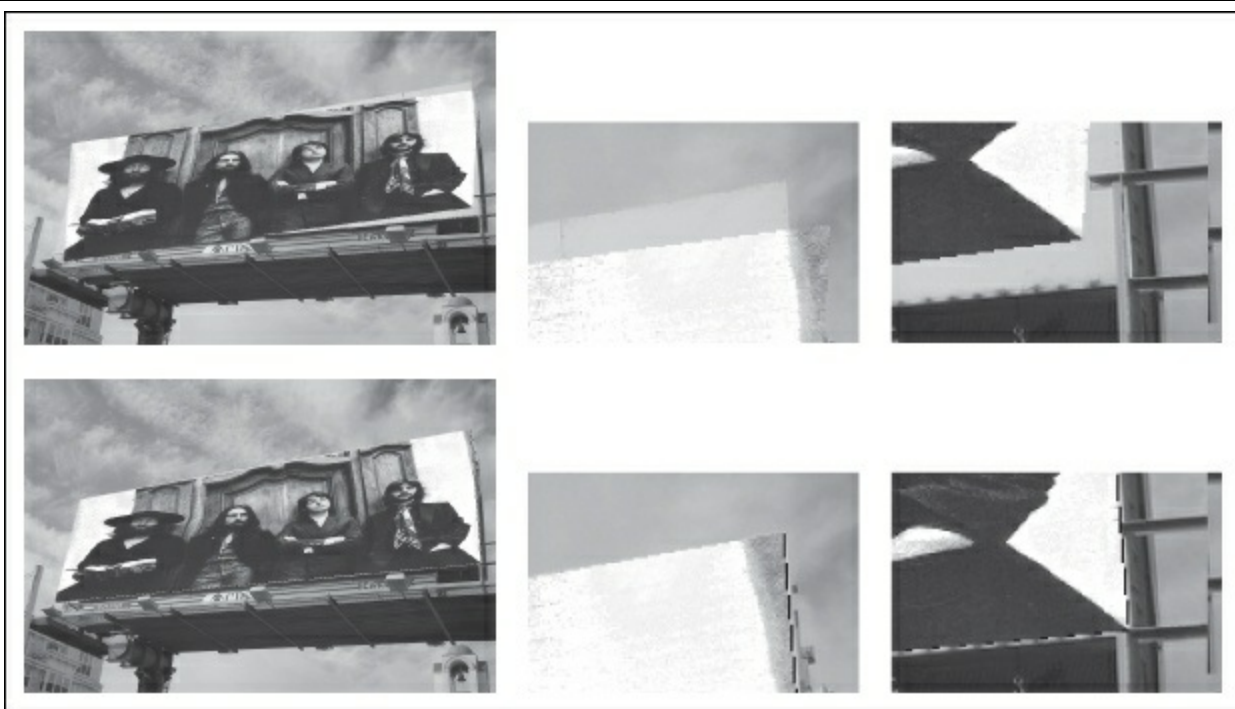
Figure 3-3. Comparing an affine warp of the full image with an affine warp using two triangles. The image is placed on a billboard with some perspective effects. Using an affine transform for the whole image results in a bad fit. The two right-hand corners are enlarged for clarity (top). Using an affine warp consisting of two triangles gives an exact fit (bottom).
