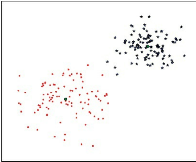
Figure 6-1. An example of k-means clustering of 2D points. Class centroids are marked as large rings and the predicted classes are stars and dots, respectively.
